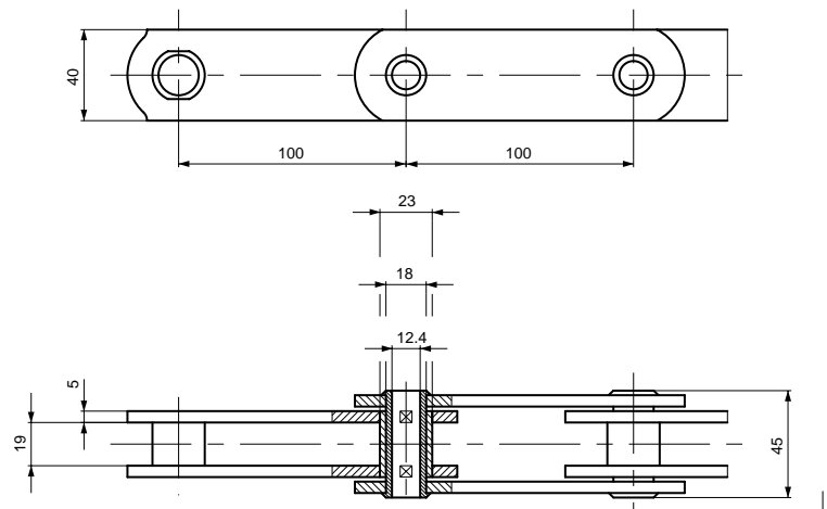
Catena P. 100x19x23 øB
